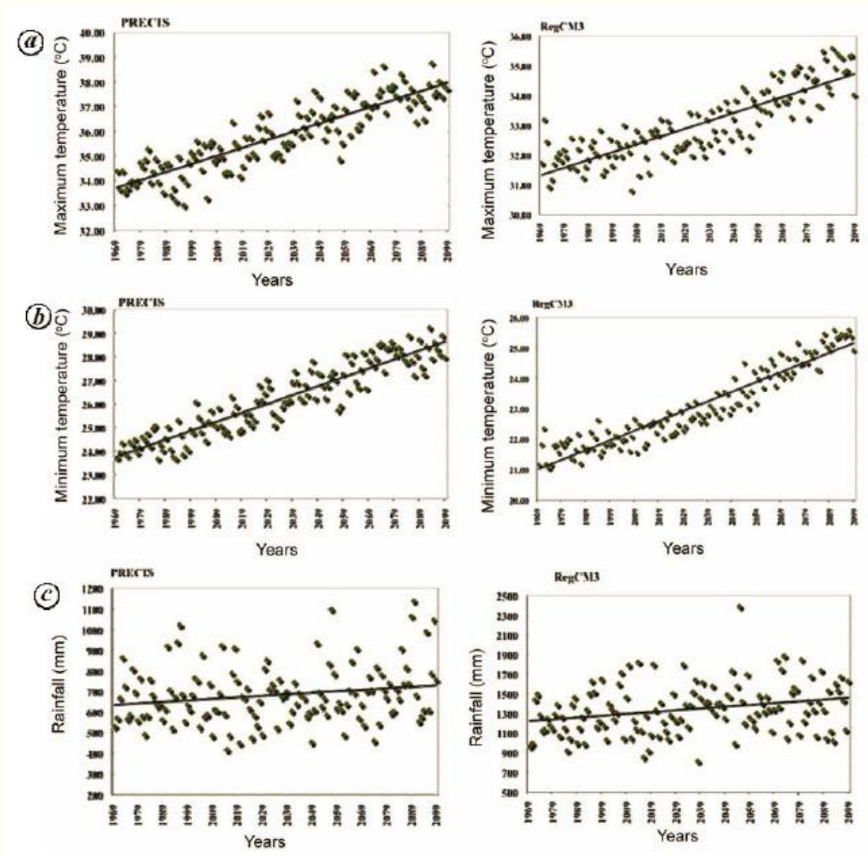
Figure 8: Temperature and rainfall projections for A1B scenario using PRECIS and
