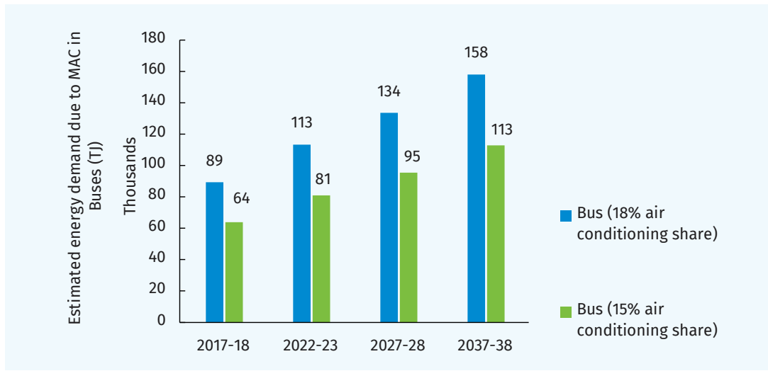
Figure 4.6: Energy Demand Projection due to MAC in Bus segment
