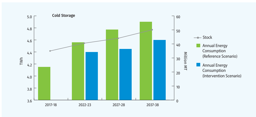
Figure 3.4: Current and Future Trends in Cold Storages
