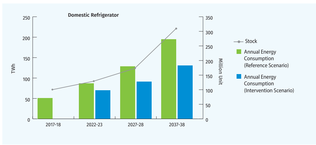
Figure 3.6: Current and Future Trends in Domestic Refrigeration
