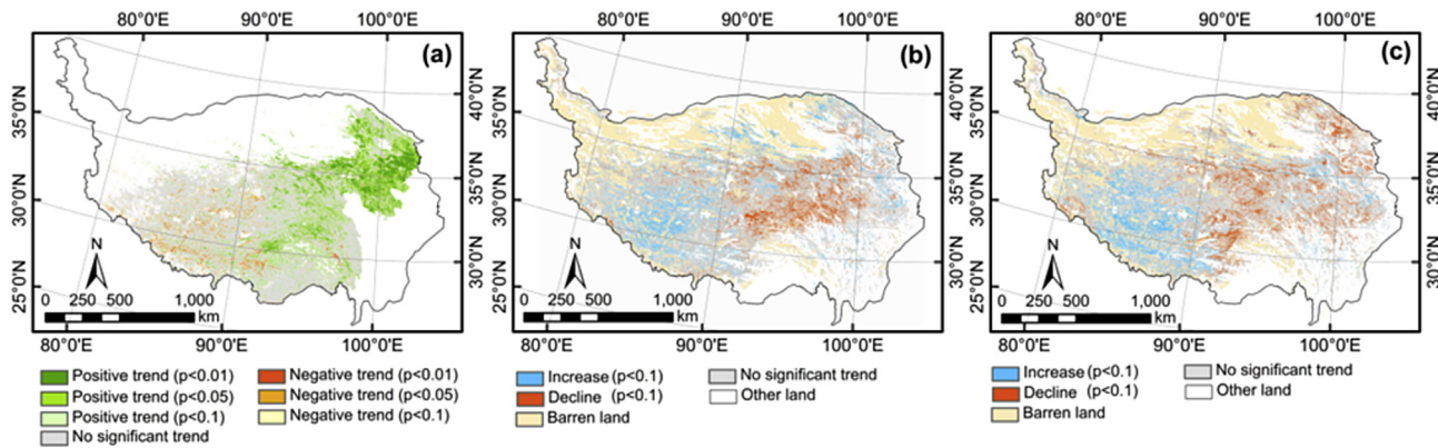
Fig. 3. Trends in (a) the growing season NDVI, (b) the start of the season, and (c) the end of the season during 2000–2009 on the Tibetan Plateau (Zhang et al., 2013; Wang et al., 2015).
