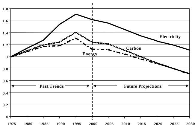
Figure 4. GDP intensities of energy, electricity and carbon for IA2 scenario (ref. 30).
