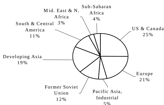
Figure 1. Per cent cumulative global CO 2 emissions from industrial sources and land-use change during 1900–1999.
