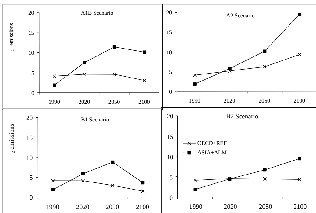
Figure 2. Fossil fuel CO 2 emissions (GtC) in industrialized and developing regions under four SRES marker scenarios. OECD90 region includes countries of the Organization for Economic Co-operation and Development as of 1990. REF region consists of countries undergoing economic reform and groups together in the East and Central European countries and the newly independent states of the former Soviet Union. ASIA region includes all developing countries in Asia (excluding the Middle East). ALM region stands for the rest of the world and corresponds to developing countries in Africa, Latin America and Middle East. Scenarios A1B, A2, B1 and B2 (ref. 29)
