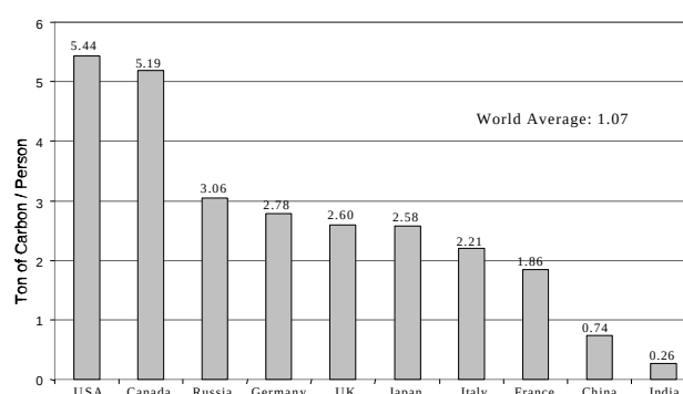
Figure 3. Per capita carbon emissions from energy for the year 2003 (ref. 27).
