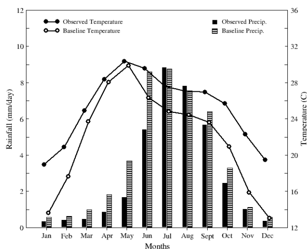
Figure 3. Observed and PRECIS-simulated (baseline, 1961–1990) mean annual cycles of all-India mean precipitation and surface air temperature.
