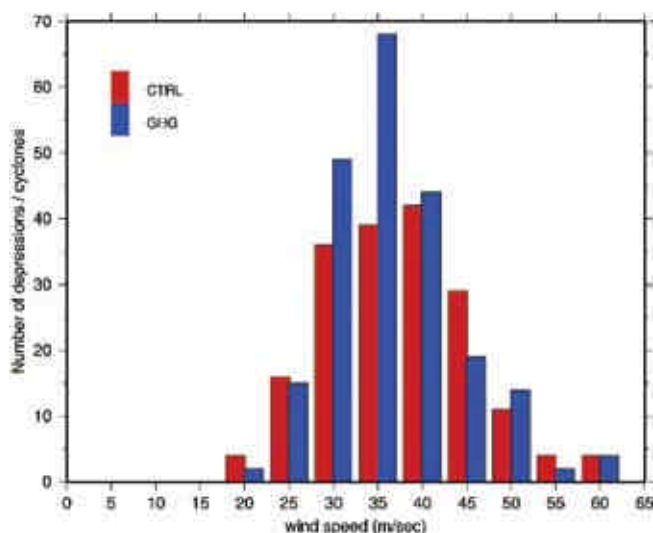
Figure 4. Frequency distribution of maximum wind speeds associated with cyclones in HadRM2 for CTRL (199s, red columns) and increased GHG (2050s, blue columns)
