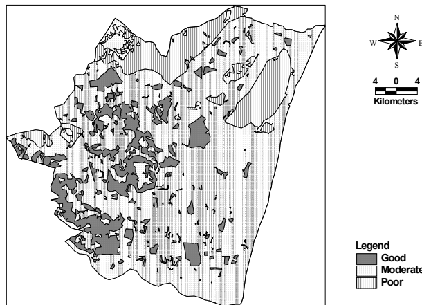
Fig. 5. Classification of areas favourable for artificial recharge
