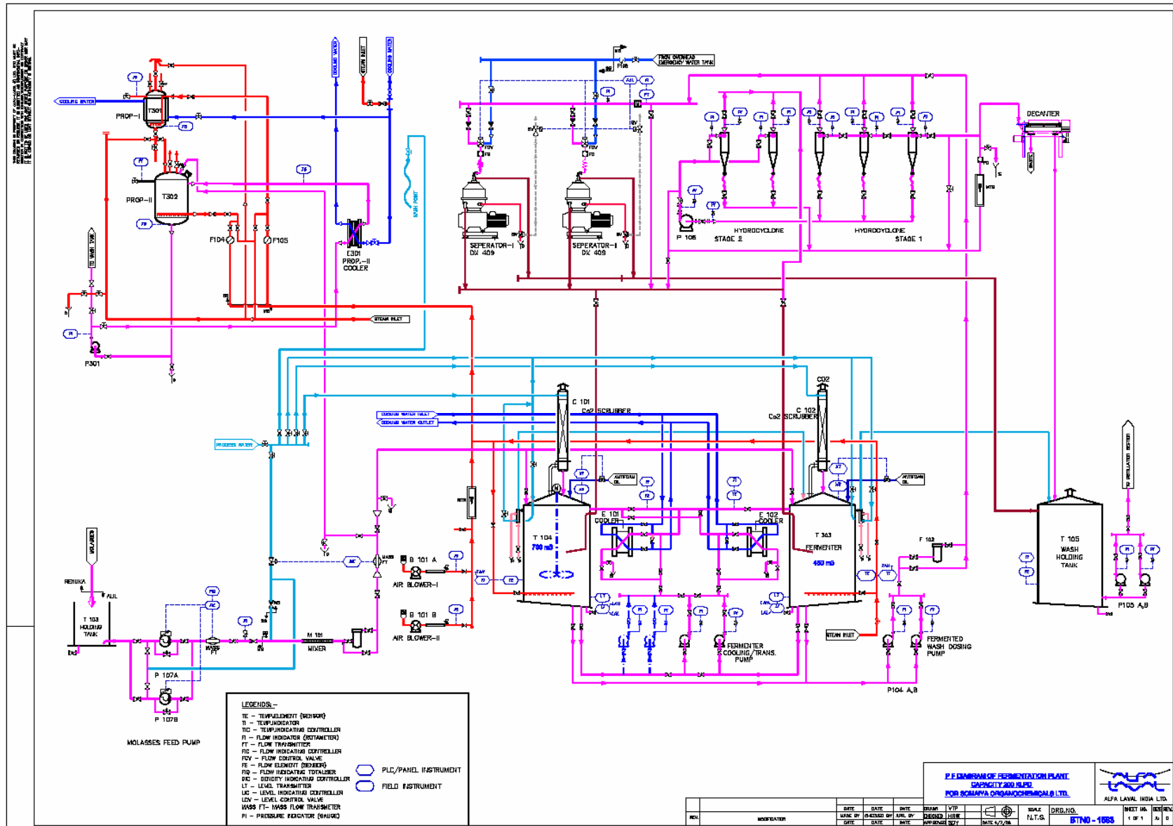
Figure 1: Process flow of Fermentation section
