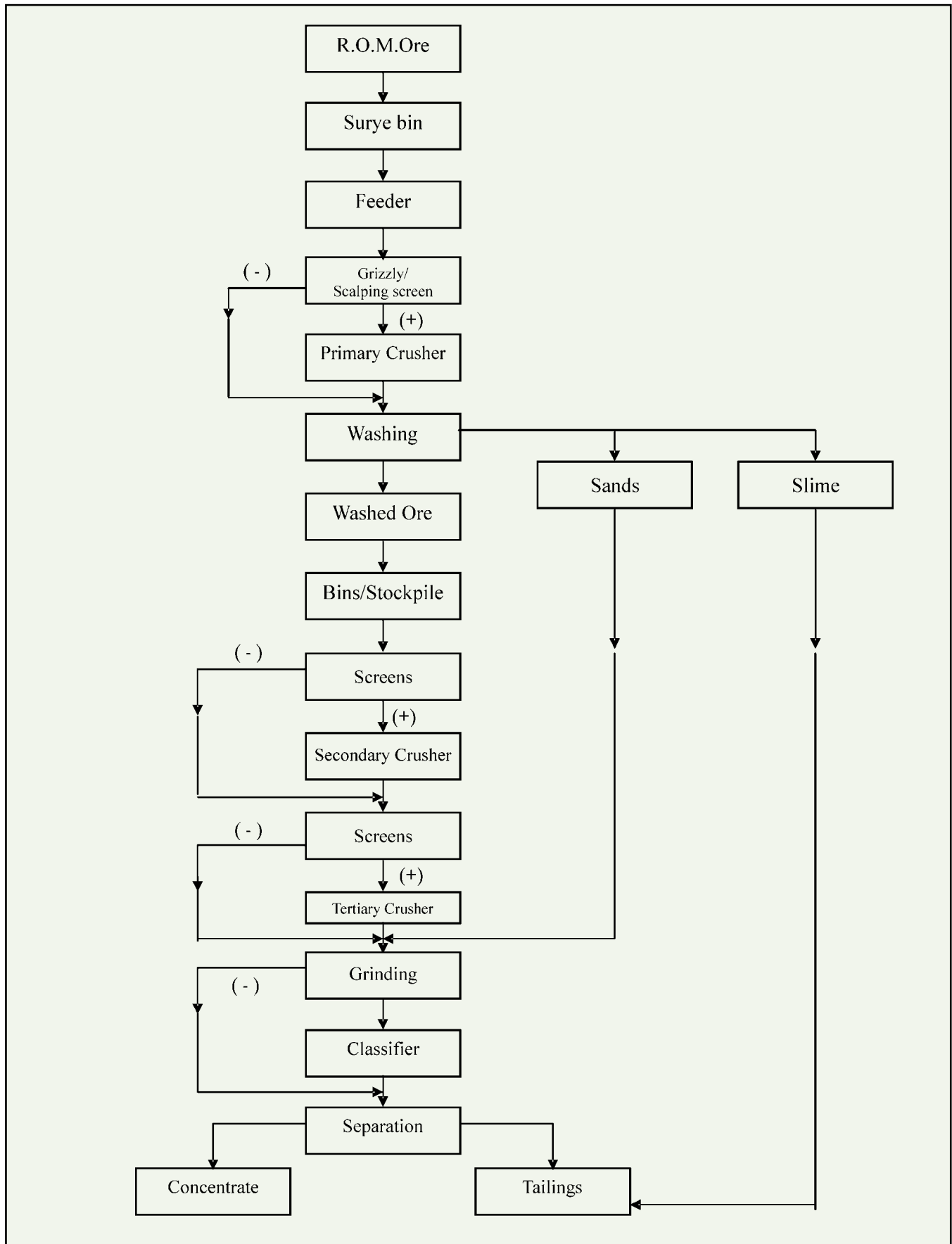
Fig1.1 Flow Chart for Ore Beneficiation Sharing Unit Operations
