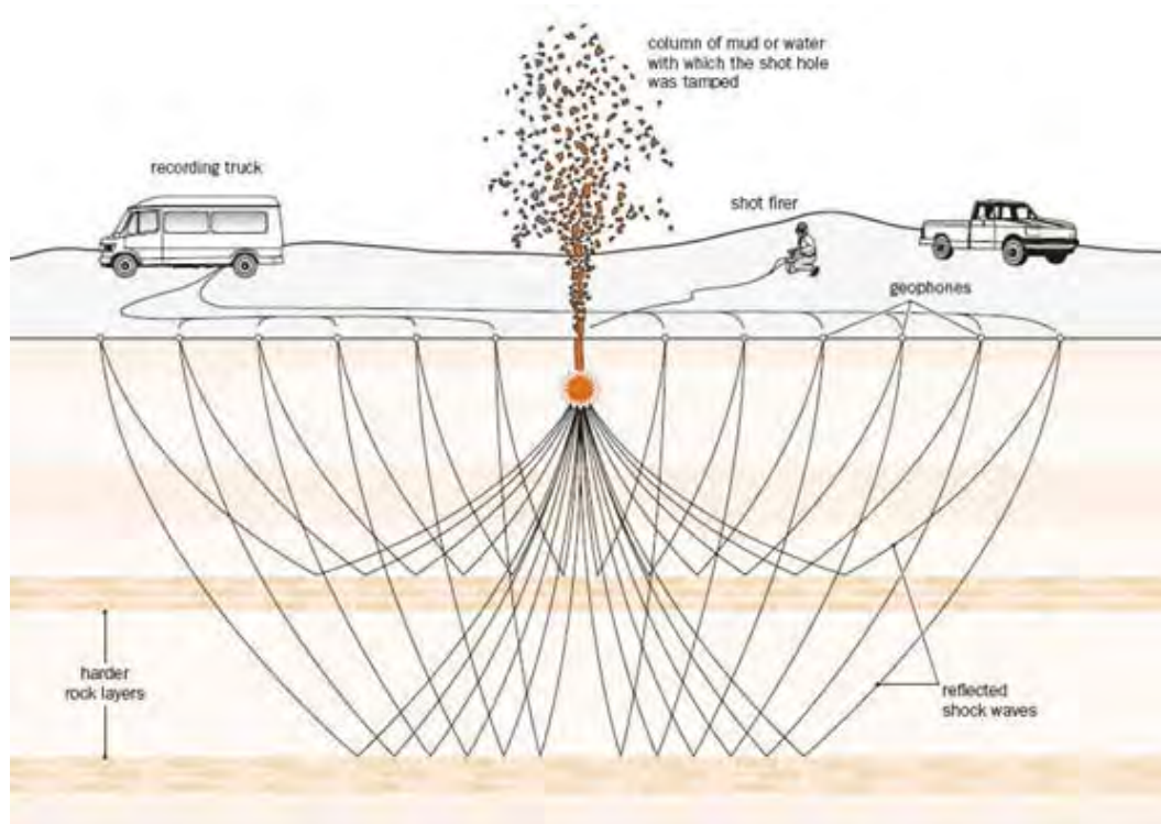
Figure 3-11: Seismic Surveys
