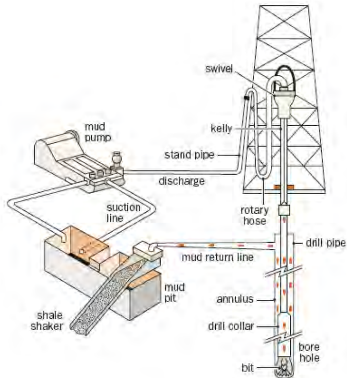
Figure 3-12: Drilling
