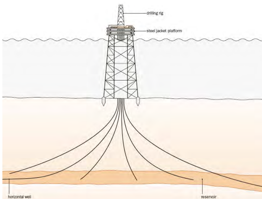
Figure 3-16: Directional Drilling
